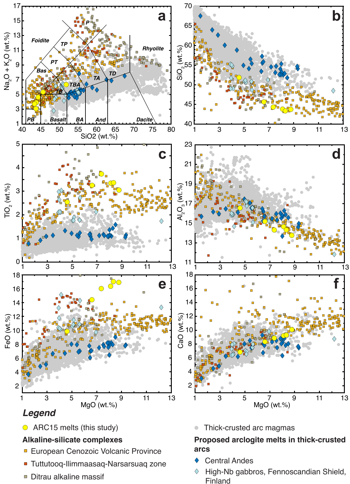
Fig. 5. Total alkali-silica diagram (a) and major element oxide-MgO diagrams (b-f) of experimental ARC15 melts compared to arc volcanics emplaced upon >40 km-thick crust (Aleutian arc, Andean arc, Cascade arc, Central American volcanic arc, Honshu arc, Izu-Bonin arc, Kamchatka arc, Kurile arc, Mexican Volcanic Belt, Sunda arc, New Zealand arc), magmas from the central Andes (Ducea et al., 2013; Murray et al., 2015) and Fennoscandian Shield (Kara et al., 2020) previously interpreted to be derived from arclogites, and magmas from alkaline-silicate complexes. ARC15 melts plot outside of the compositional field of thick-crusted arc magmas but overlap with alkaline-silicate complexes. Arclogite melting is therefore not a dominant source of magmatism at thick-crusted arcs but may contribute significantly to the formation of alkaline-silicate complexes. Abbreviations in (a) are as follows: PB = picro-basalt, BA = basaltic andesite, And = andesite, TB = trachy-basalt, BTA = basaltic trachy-andesite, TA = trachyandesite, TD = trachydacite, Bas = basanite, PT = phono-tephrite, TP = tephri-phonolite. (For interpretation of the references to colour in this figure legend, the reader is referred to the web version of this article.)
